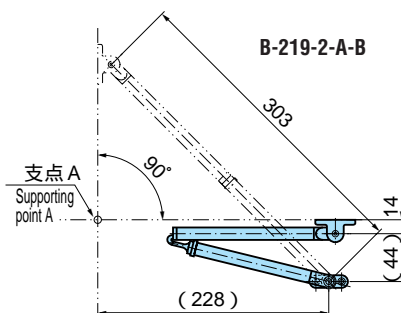
参考作動例 Example of operation (reference)
