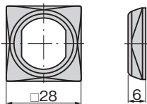
止め金回転角度90° Stopper plate turning angle
