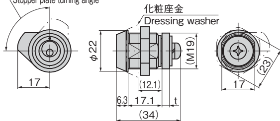
止め金回転角度90° Stopper plate turning angle
