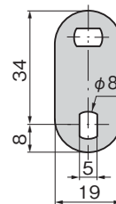
板厚 t=3.2 Plate thickness
