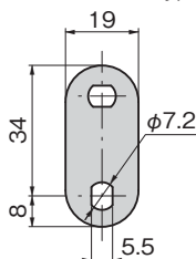
板厚 t=2.3 Plate thickness
