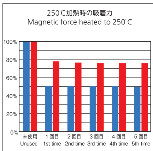
C-1100-H-2 吸着減磁率参考値 Demagnetizing factor reference values
