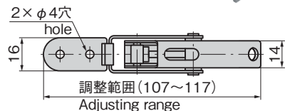
[C-1229-1・C-229-1]
