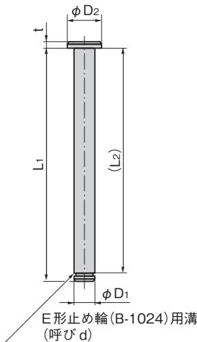
Groove for E-shaped retaining ring (nominal d)
