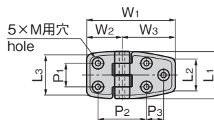
BP-19-2-2-S 皿ねじ用 For countersink screw
