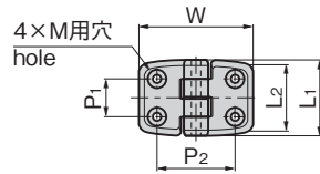
BP-19-1-2-S 皿ねじ用 For countersink screw
