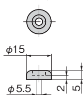
[座金] Washer
