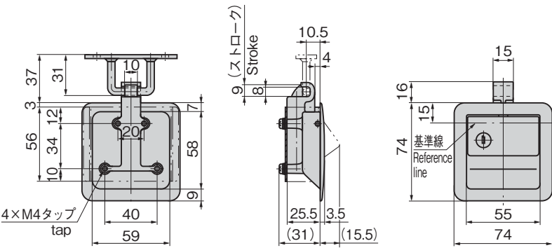
〔取付け金具〕 Installation fitting
