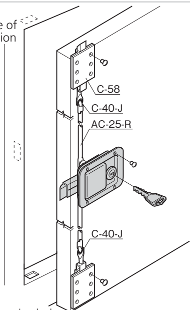
3点締め 3-point securing lock
