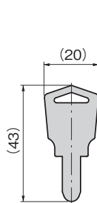
止め金(兼用型) Stopper plate (combined-use type)
