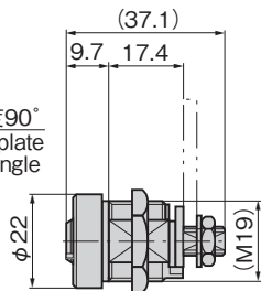
板厚 t=2.3 Plate thickness
