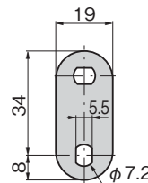
板厚 t=2.3 Plate thickness
