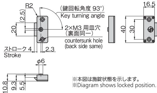
C-480-2 解錠キー型 Keep-unlocked type
