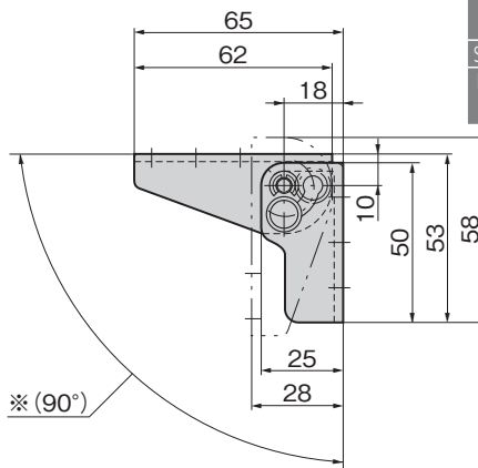
取付け参考例 Example of installation
