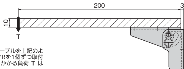
取付け参考例 Example of installation
