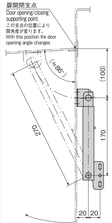
参考作動例 B-1223-11 Example of operation
