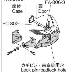
庫内安全押棒 Inside safety pushrod
