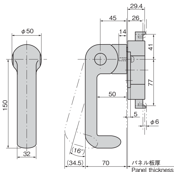
取付け例 Example of installation
